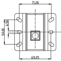
Wandmontage
