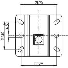
Wandmontage
